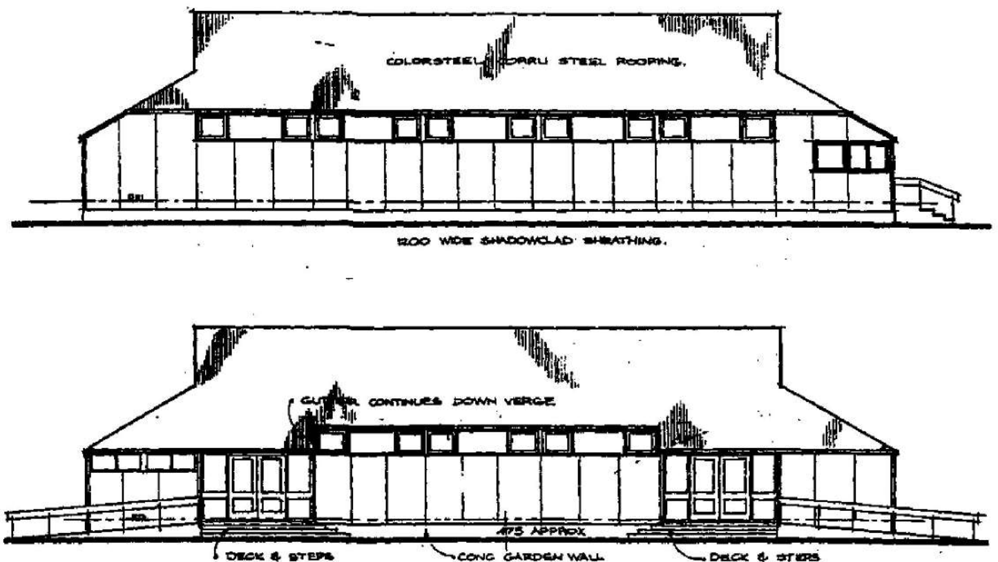
Elevation sketches of the proposed Kimihia School assembly hall.
