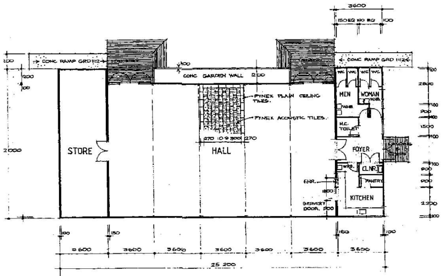
Floor plan of the proposed school assembly hall - the finished building was a flipped-image of this sketch.
