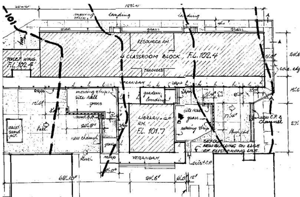
Site Plan of the new classroom block.
